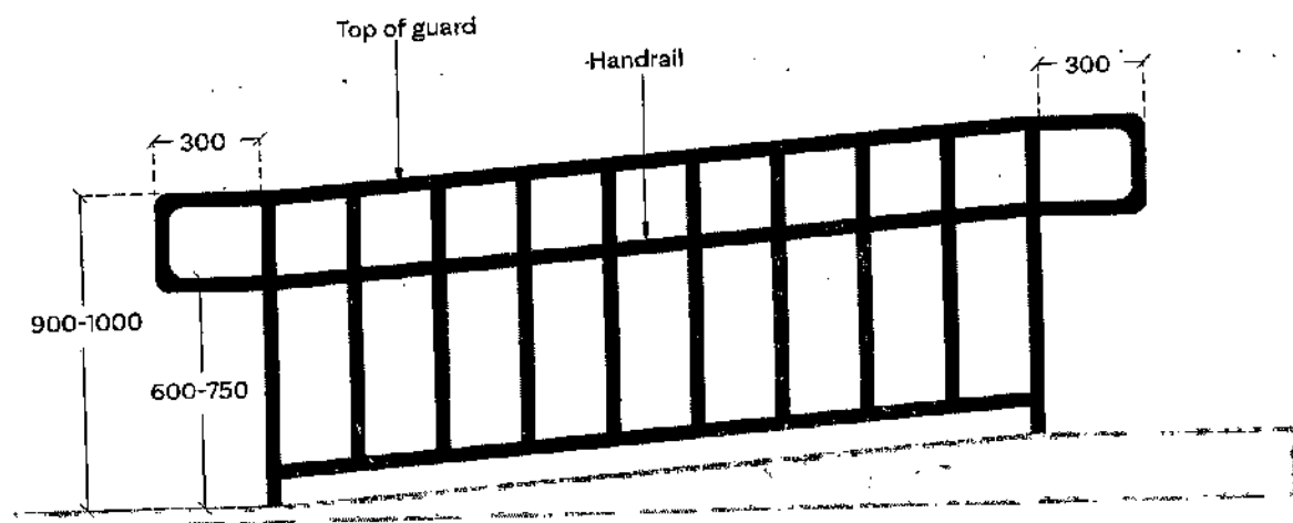
Figure 3.17 Handrail detail
