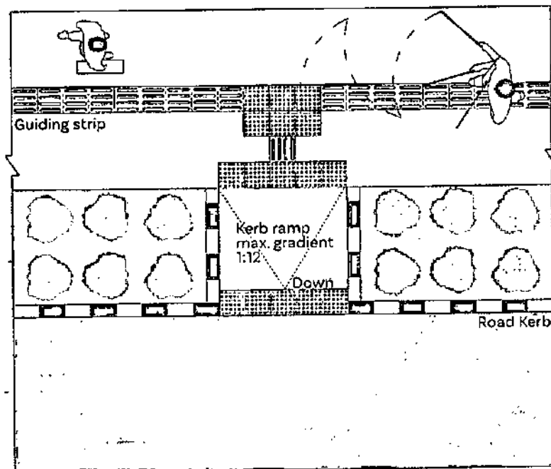
Figure 3.11 Accessible kerb ramp: Typical detail A
