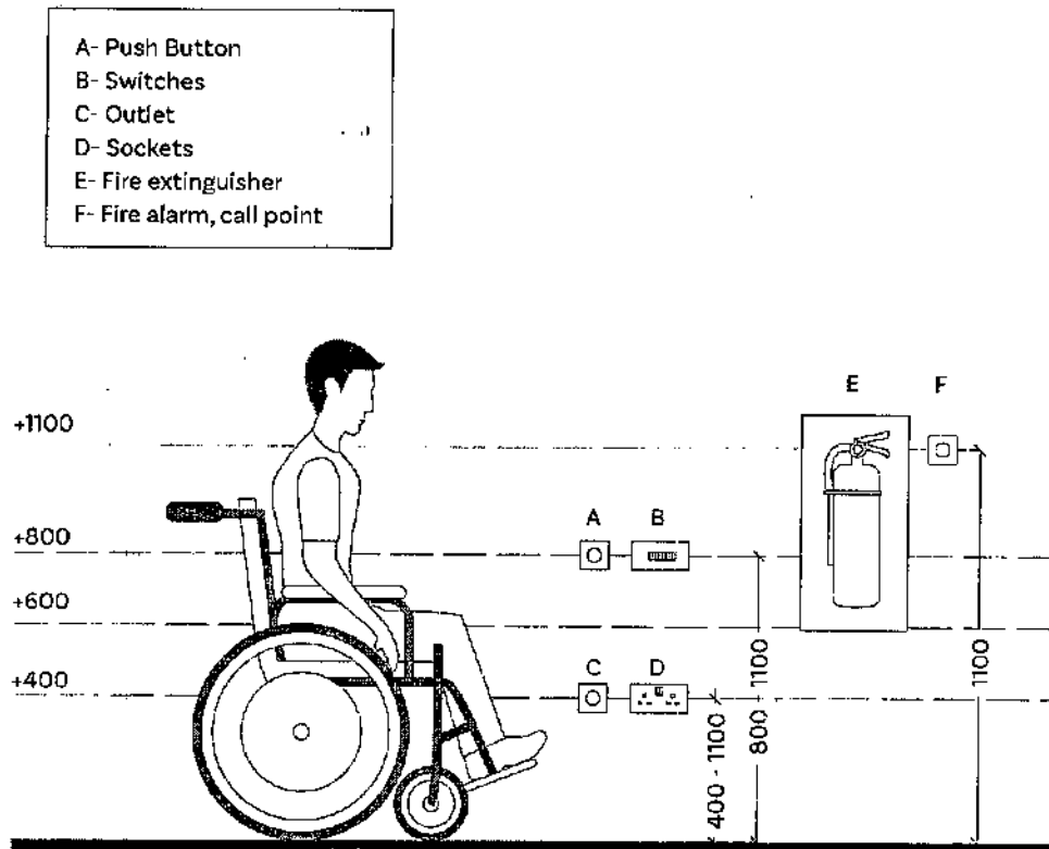
Figure 4.47 Electrical controls mounting details
