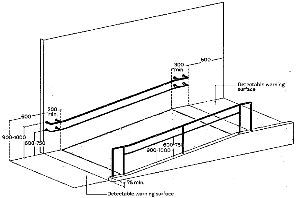
Fig a. Handrail returns to wall
