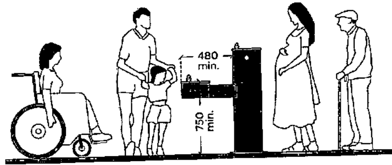
Fig a. Drinking water fountain heights (Side Elevation)
