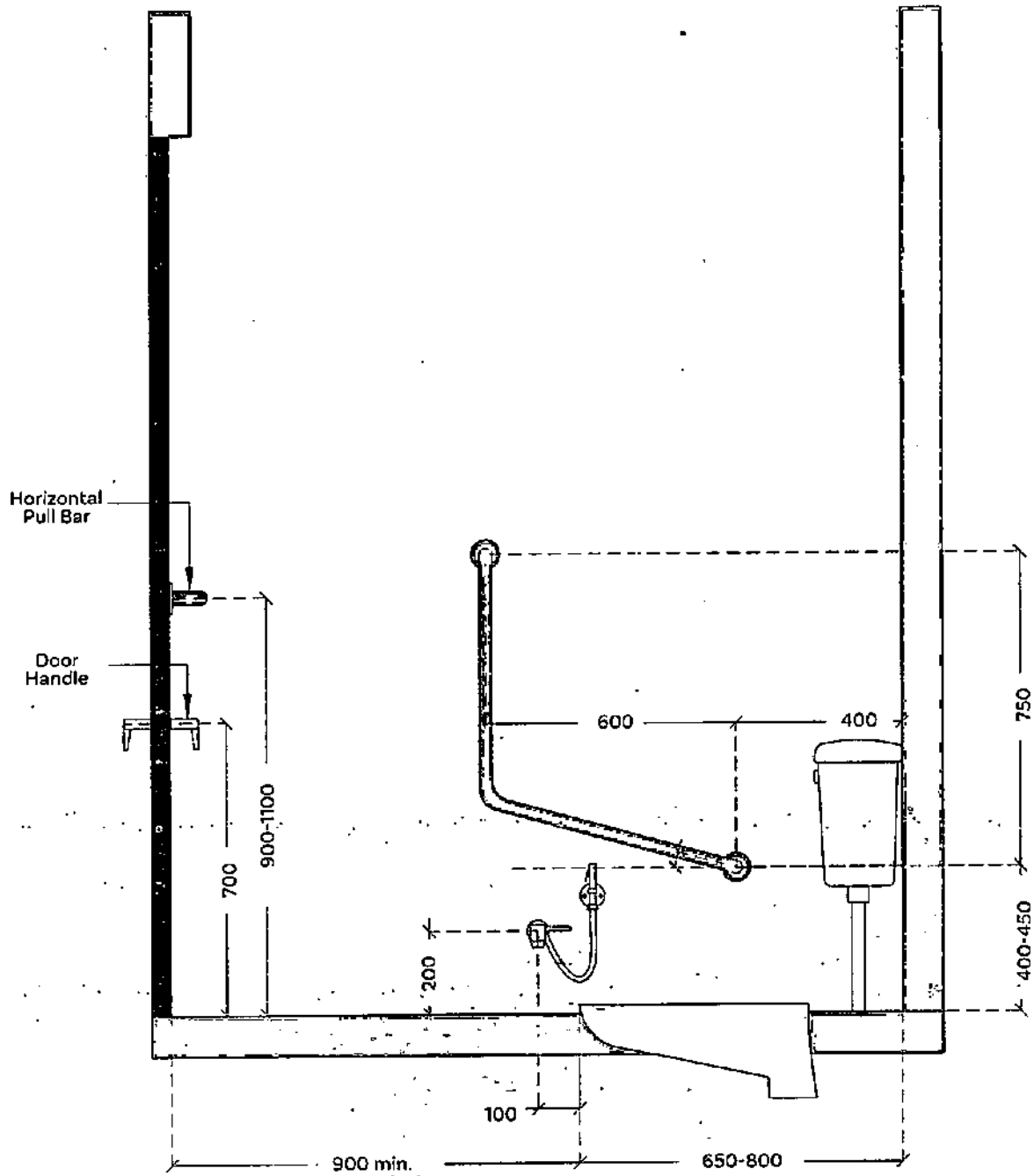
Figure 4.35 Ambulant Indian Toilet detail: Sectional elevation type B
