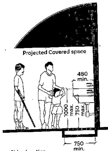
Fig a. Drinking water fountain heights: Elevations Figure 3.24 Outdoor water fountain
