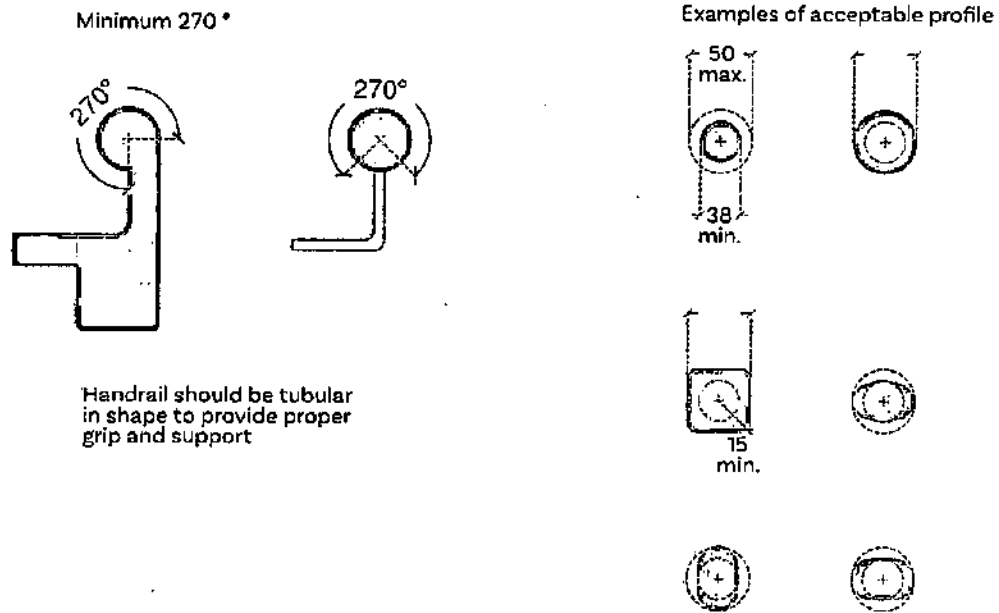
Fig a. Handrail cross-sectional profile
