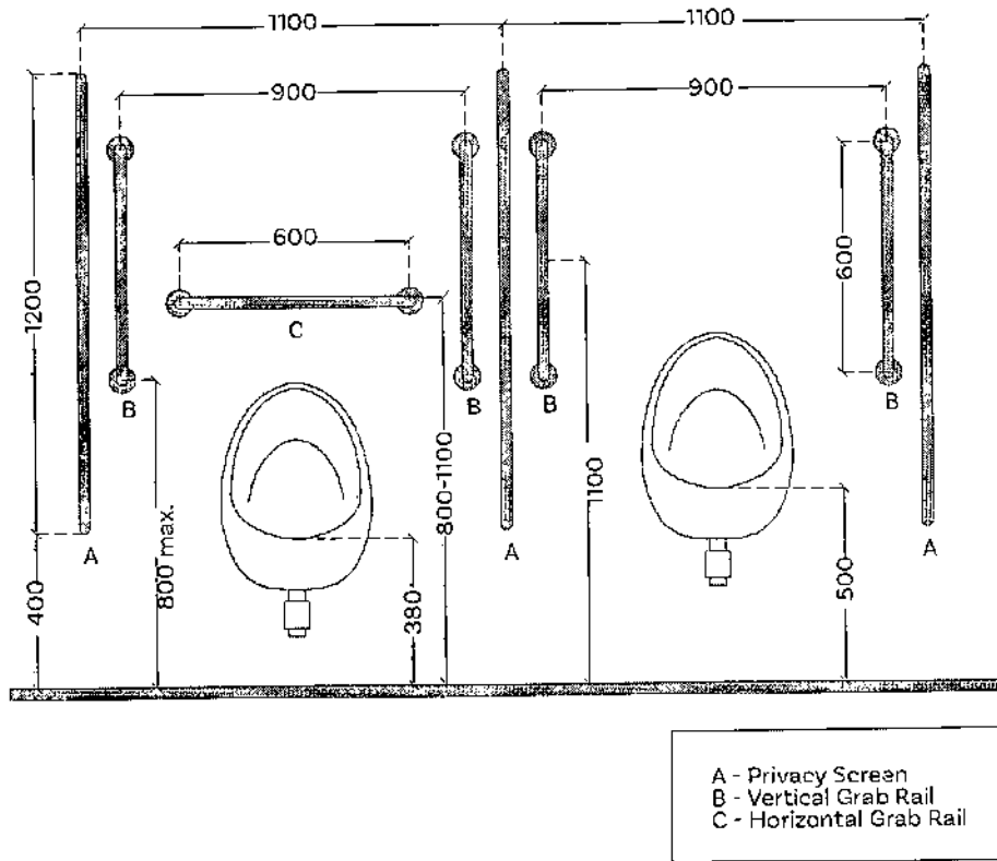
Fig a: Accessible urinal: Sectional elevation
