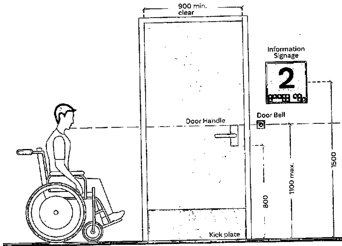
Figure 4.44 Door details
