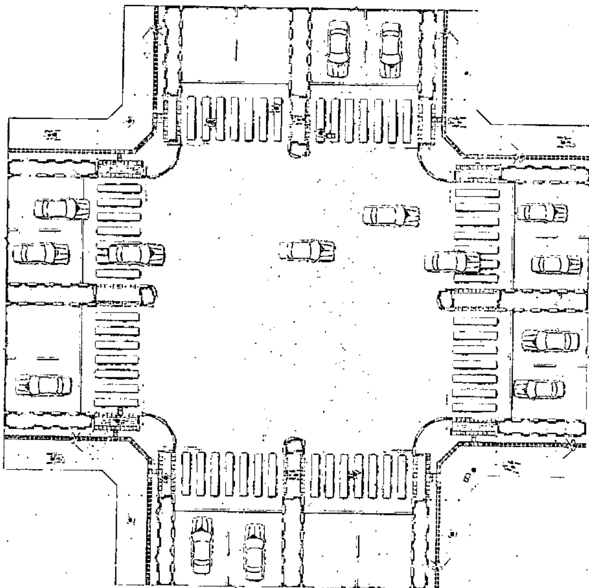
Figure 6.2 Road Intersection with accessible features
