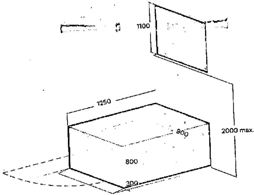
Figure 4.19 Platform lift
