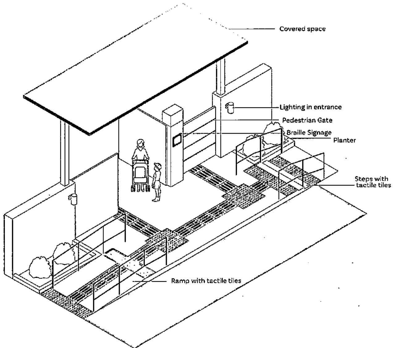
Figure 3.1 Accessible site entrances: Typical detail A
