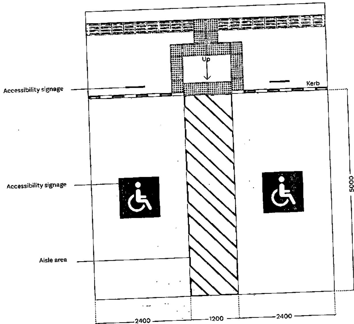
Figure 3.7 Typical accessible car parking unit: Type B
