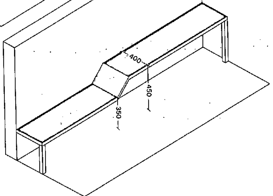
Figure 3.29 Accessible seating typologies: 3d visualization Type B
