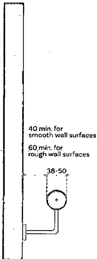
Fig b. Handrail clearance from the wall
