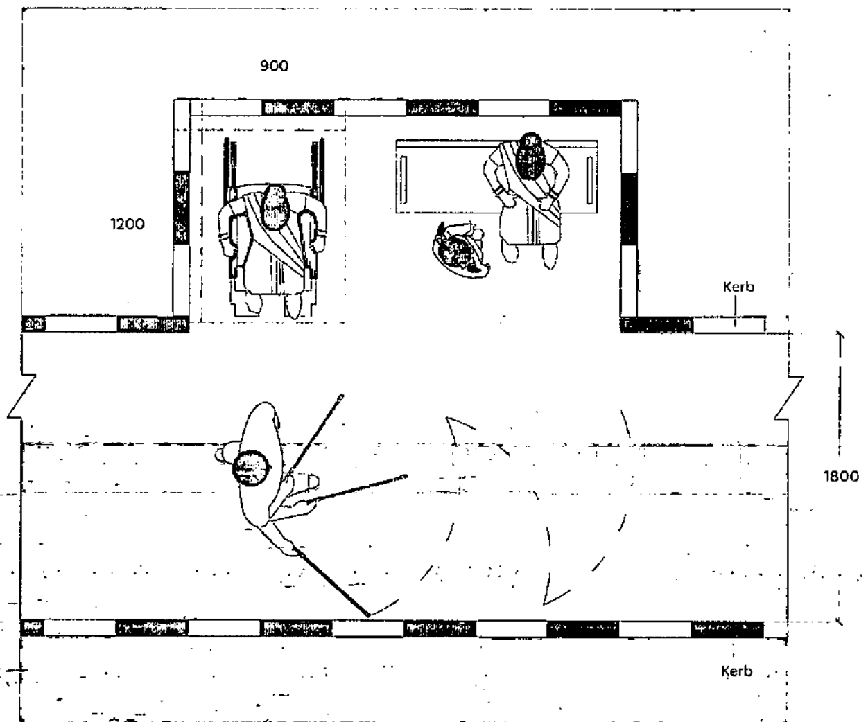
Figure 3.39 Dimension and space requirement for seating in parks and green spaces
