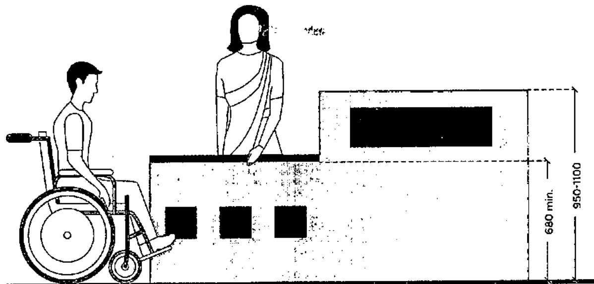
Figure 4.2 Reception counter with accessible heights
