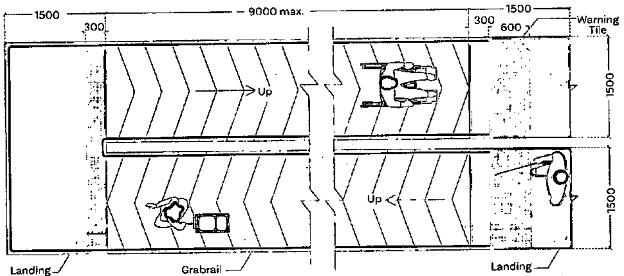
Figure 4.9 Typical details of 'U' Shaped ramp
