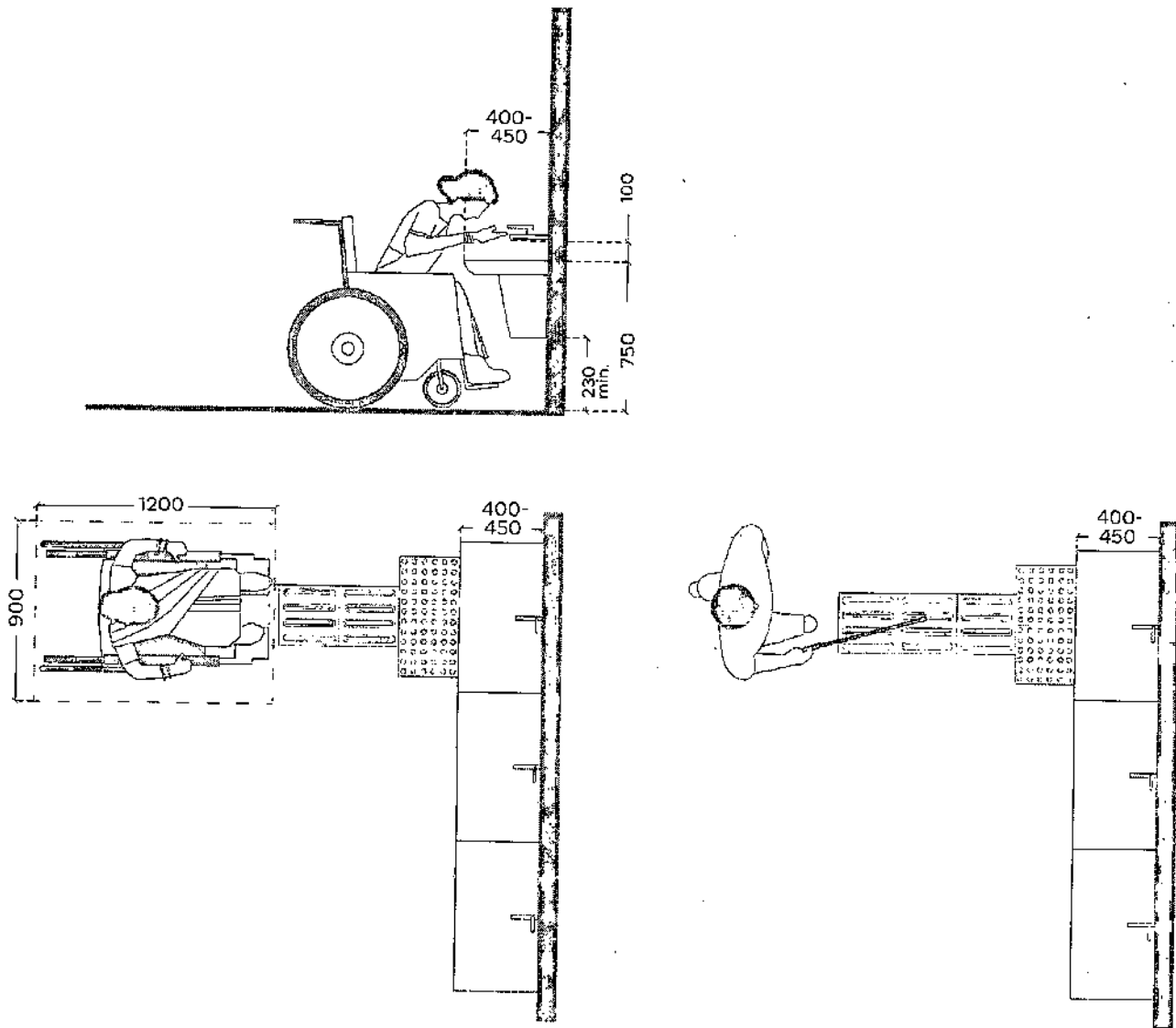
Figure 4.21 Typical layouts for accessible drinking water fountain
