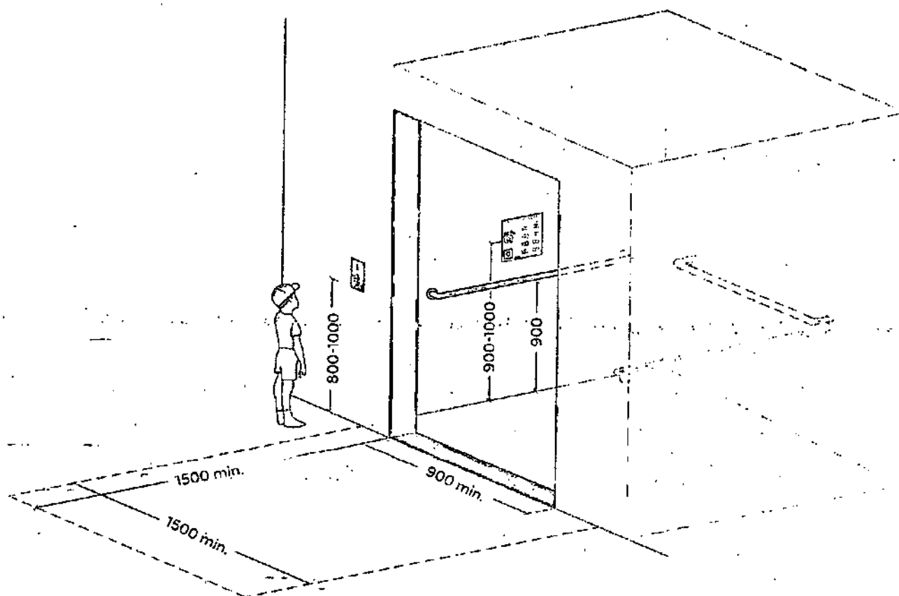
Figure 4.18 Lift platform dimensions
