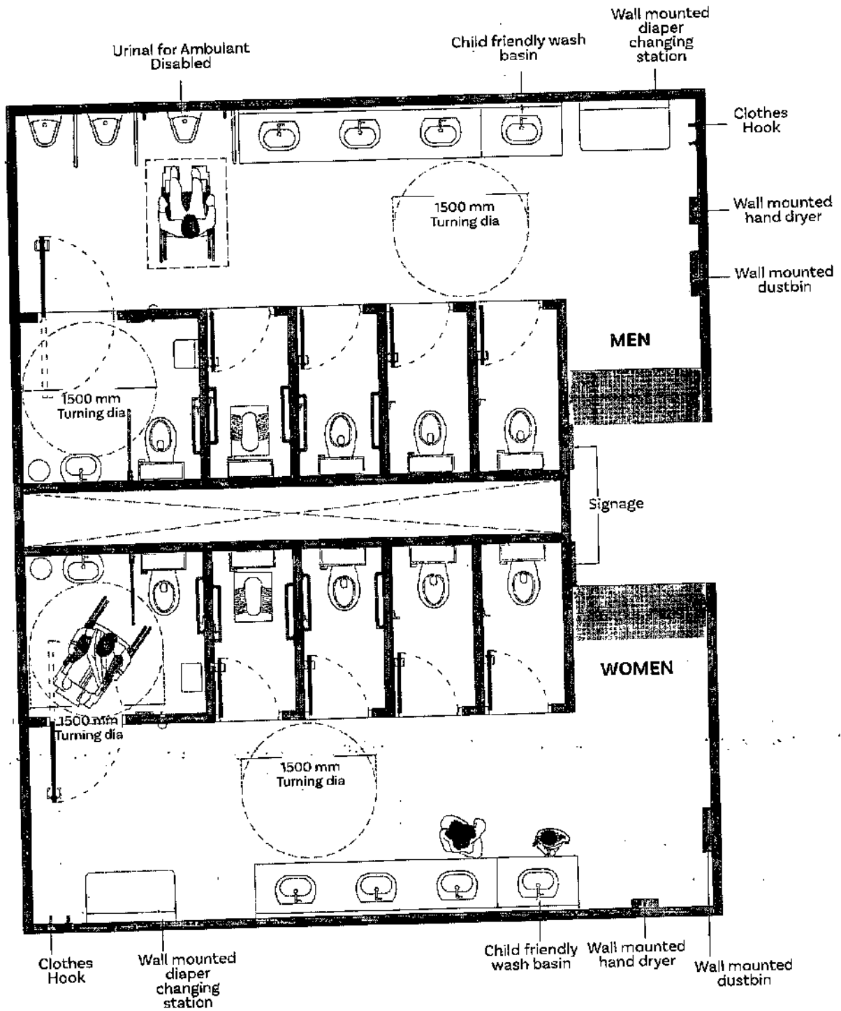
Figure 4.22 Accessible public toilet layout: Type A
