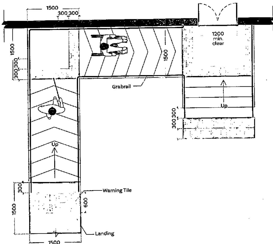
Figure 4.10 Typical details of 'L' Shaped ramp with steps: Type A
