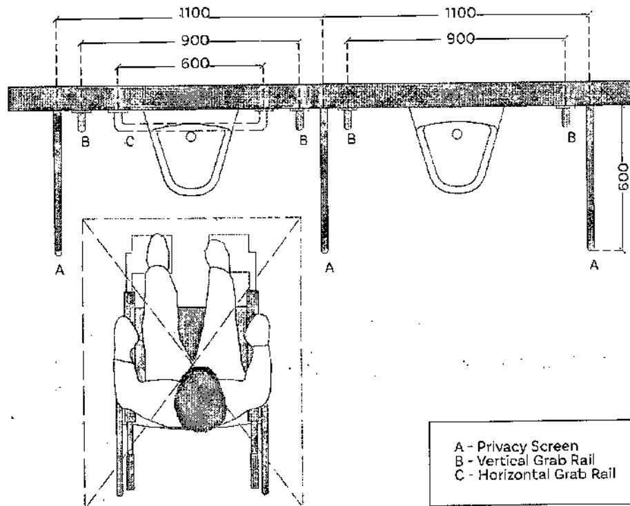
Fig b: Accessible urinal: Plan layout
