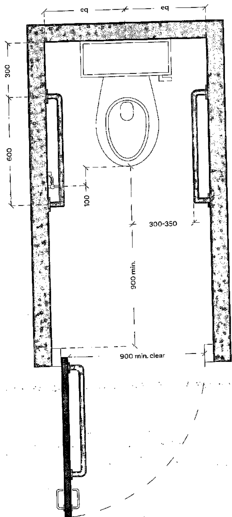
Figure 4.31 Ambulant Toilet detail: Plan Layout
