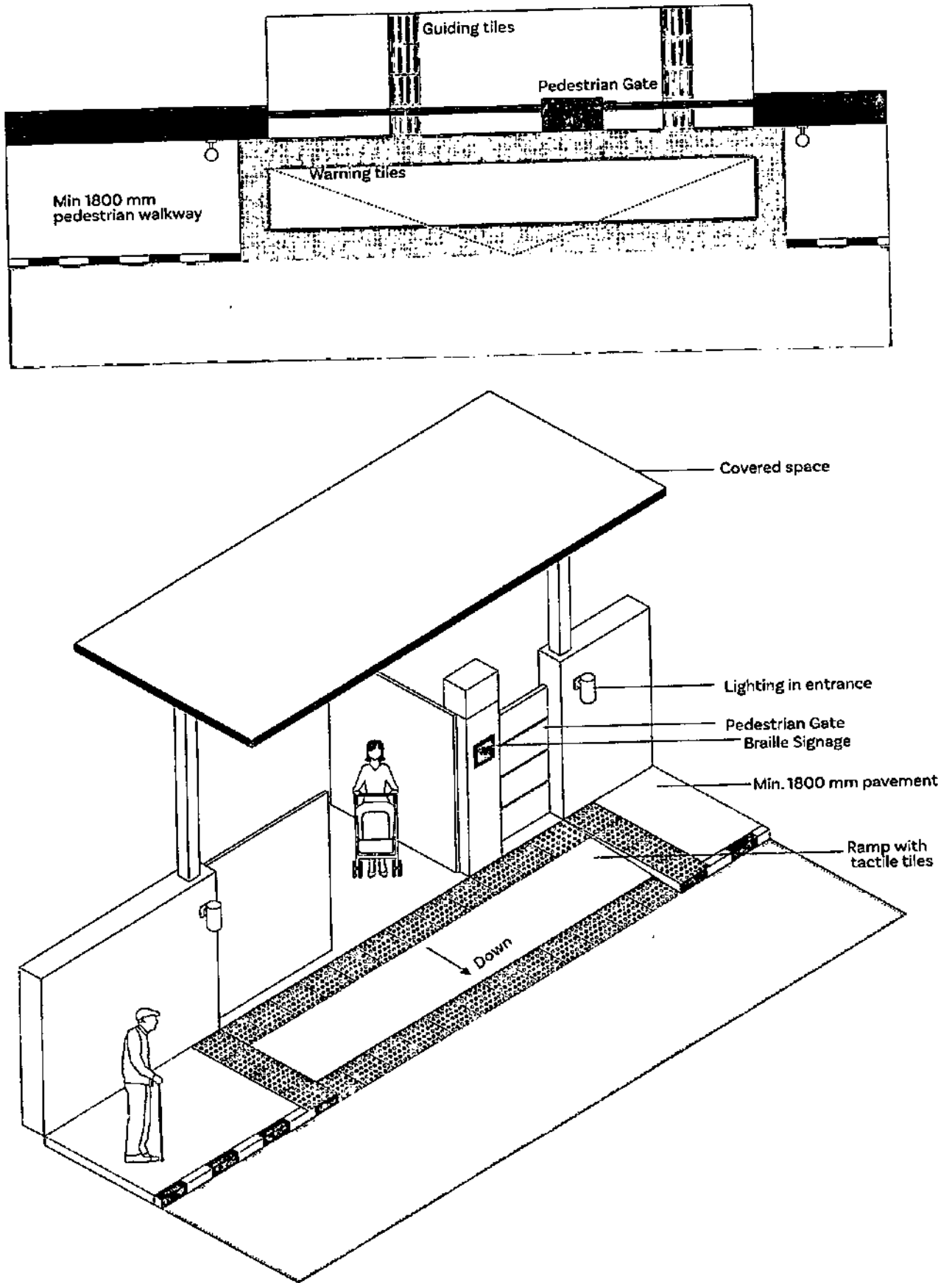
Figure 3.2 Accessible site entrances: Typical detail B
