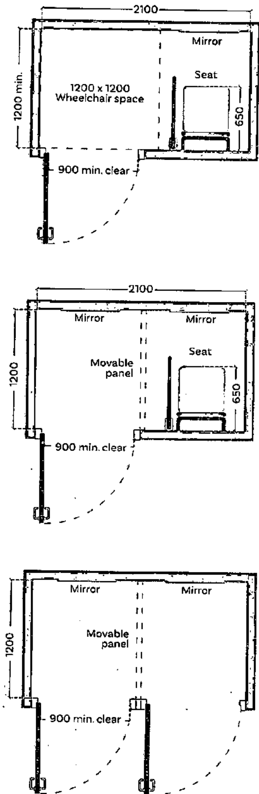
Figure 4.38 Changing room with seat details
