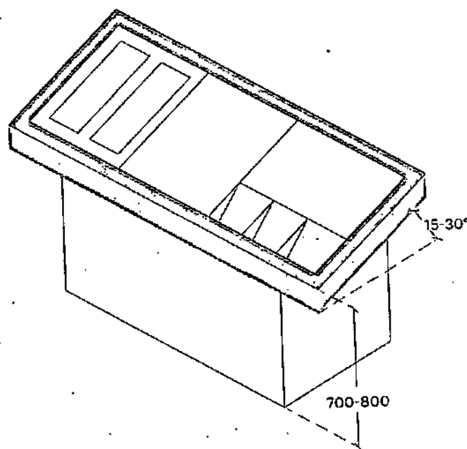
Figure 5.1 Information Display Counter
