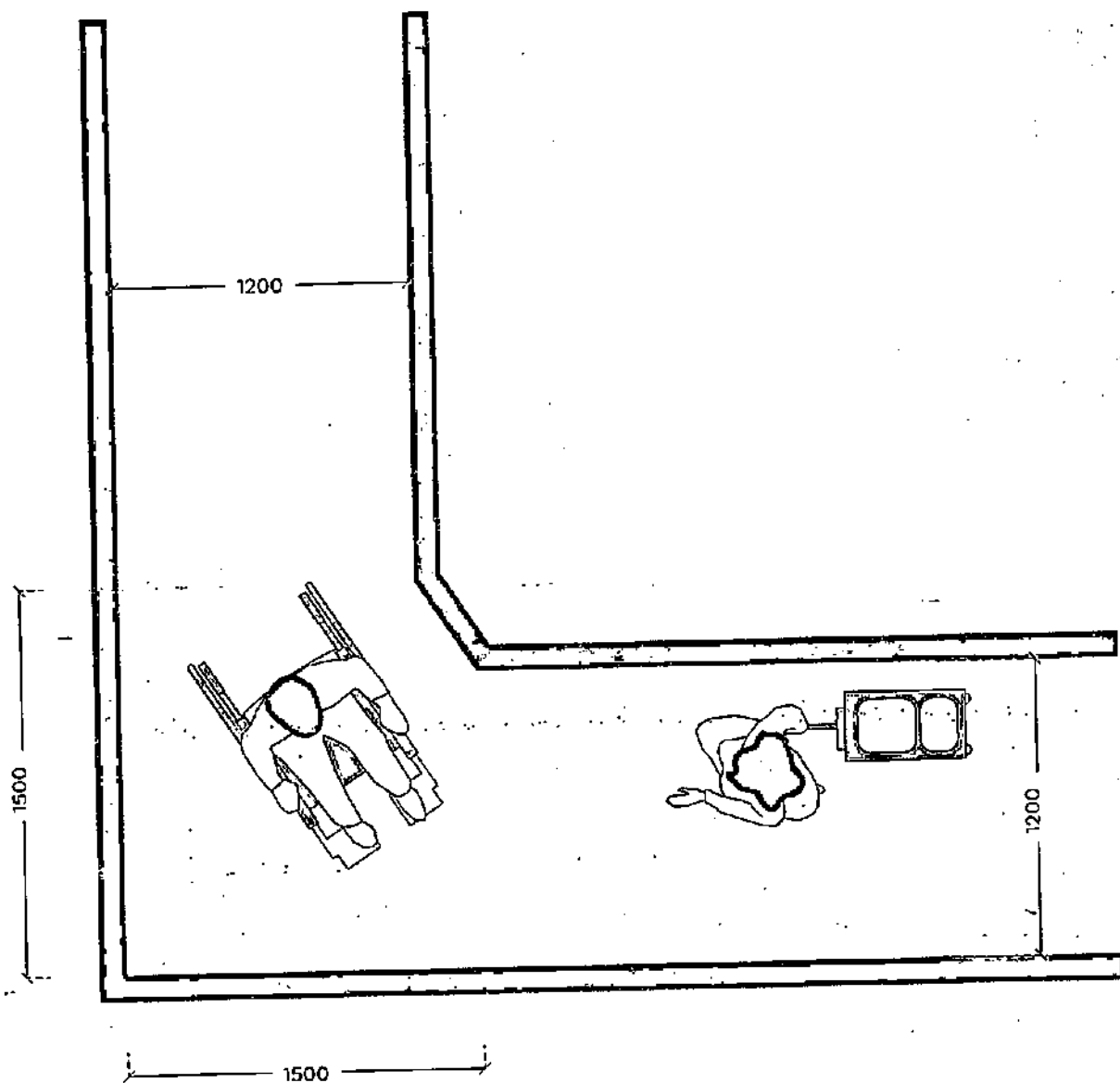
Figure 4.4 Dimension and space requirement for right-angled accessible corridor
