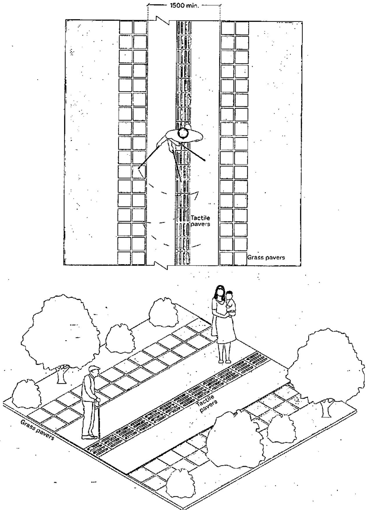
Figure 3.38 Accessible paved pathways with grass pavers
