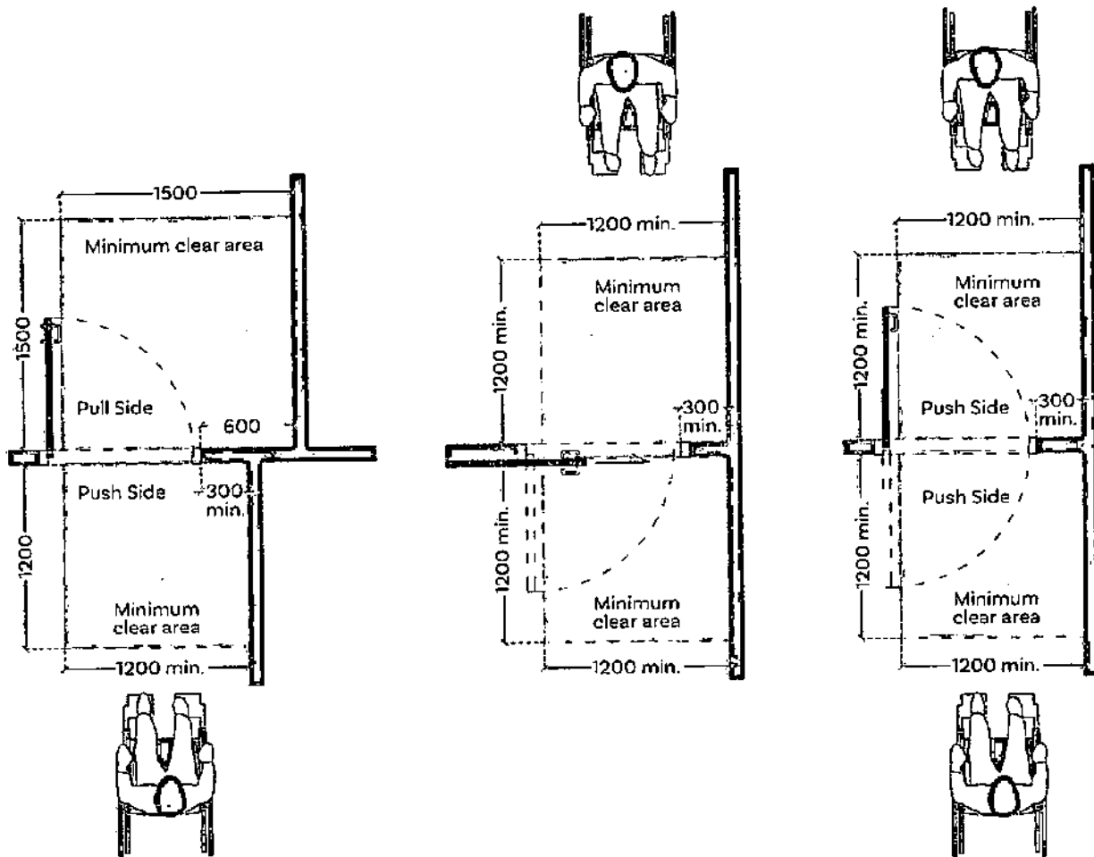
Fig c: Case of both-side push swinging doors
