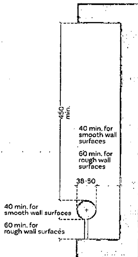
Fig c. Handrail in recess
