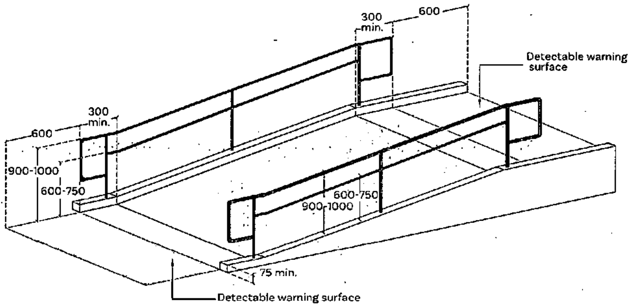
Fig b. Handrail returns to post
