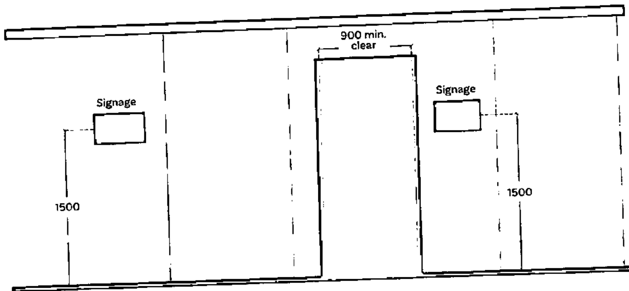
Figure 5.2 Height and placement of signages
