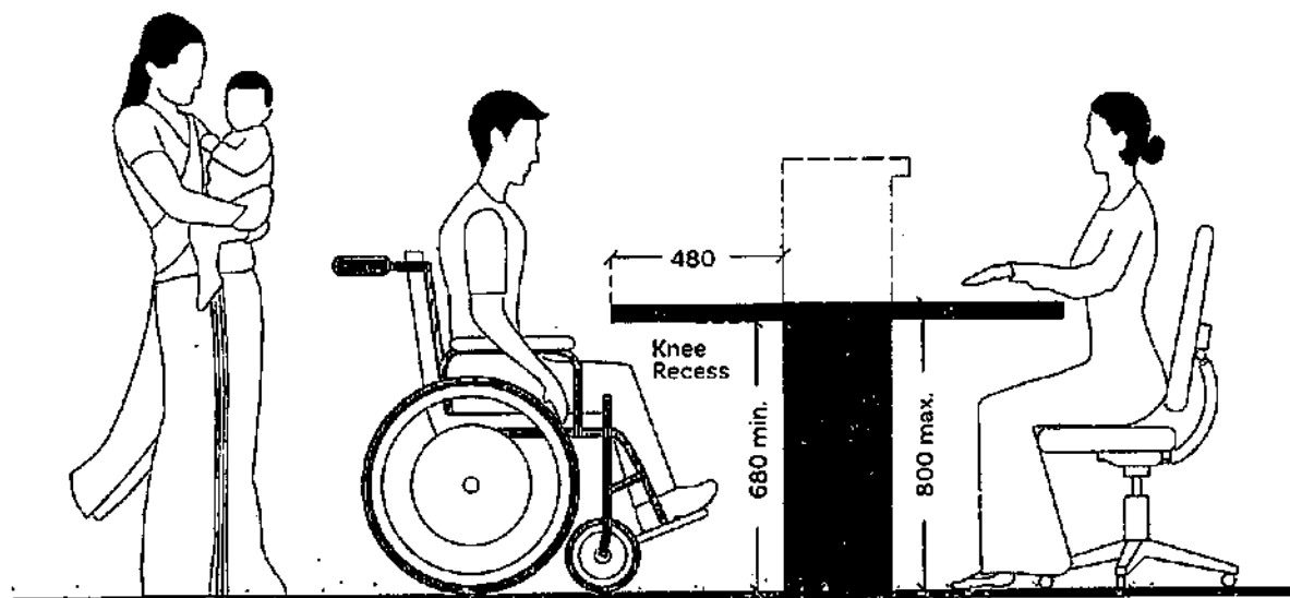
Figure 4.3 Accessible Service and Information Counters
