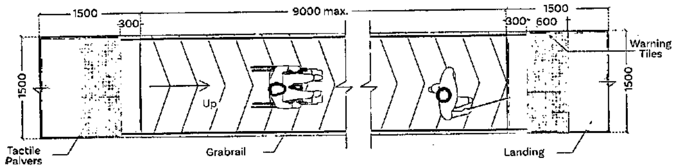
Figure 4.8 Typical details of Straight ramp
