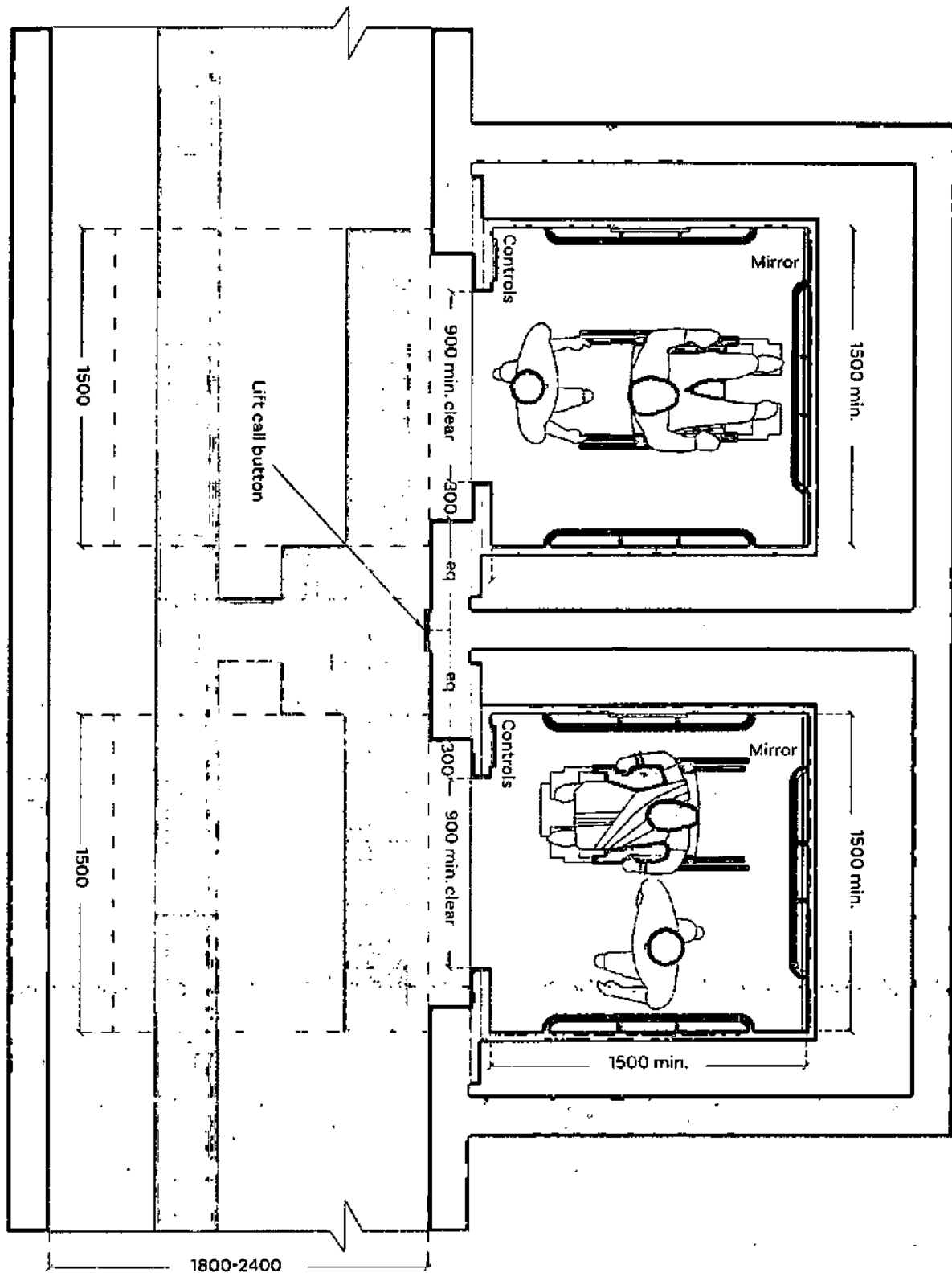
Figure 4.14 Accessible lift cars in parallel layout
