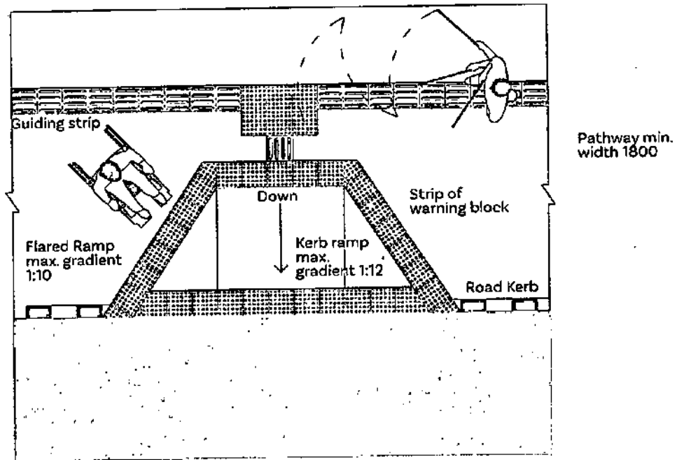
Figure 3.12 Accessible kerb ramp: Typical detail B
