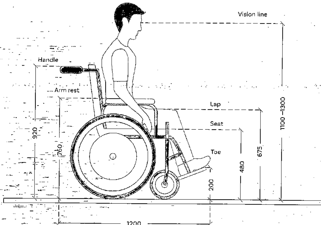
Figure 2.8 Wheelchair dimensions
